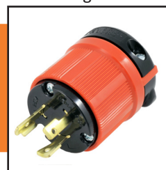
ASL630P NEMA L6-30P Replacement Plug.
