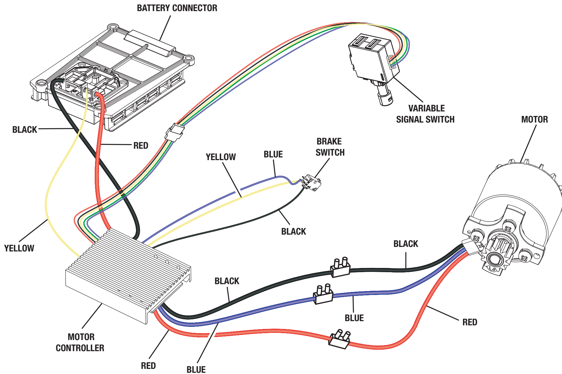
WIRING DIAGRAM
