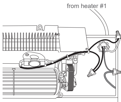
Figure 8 Heater #2
