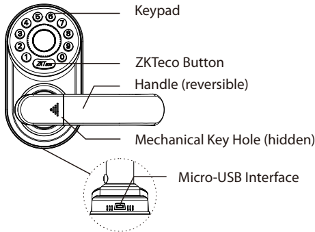
Outdoor Assembly
