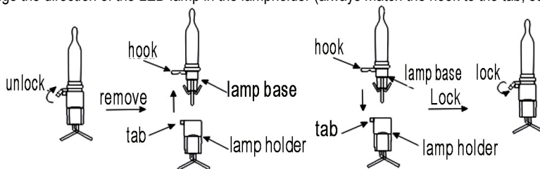
Fig. 1 Unlock and remove the burned out lamp
