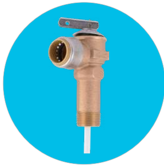
Cash Acme® Temperature & Pressure Relief Valves Designed for the protection of the water heater against excess pressure and temperature.
