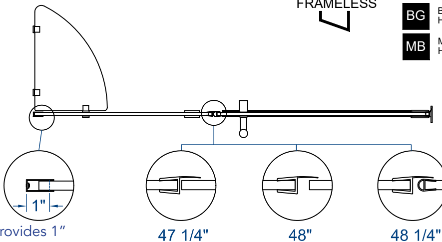
DOOR GAP AT DIFFERENT OPENING WIDTHS
