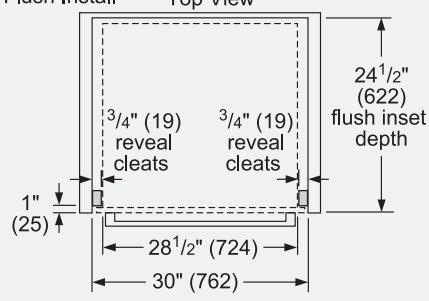
Flush Install Top View
