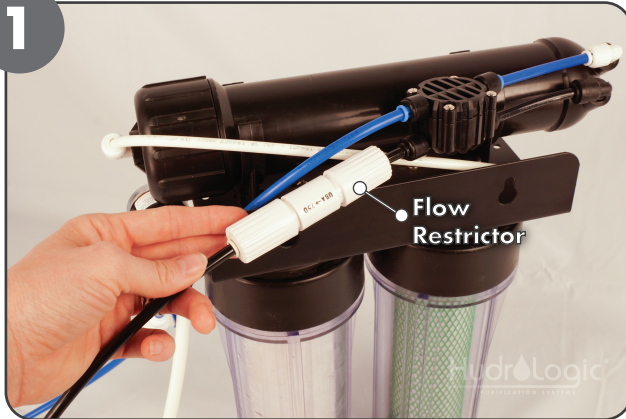
Remove flow restrictor
