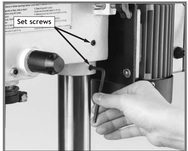
Figure 11. Securing the headstock to the column.
