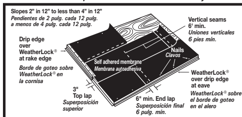
Fig. 2B Underlayment – Low Slope Membrana impermeabilizante – Pendiente baja
