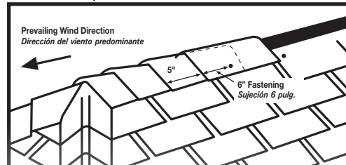
Fig.8 Hip & Ridge Limatesa y cumbrera
