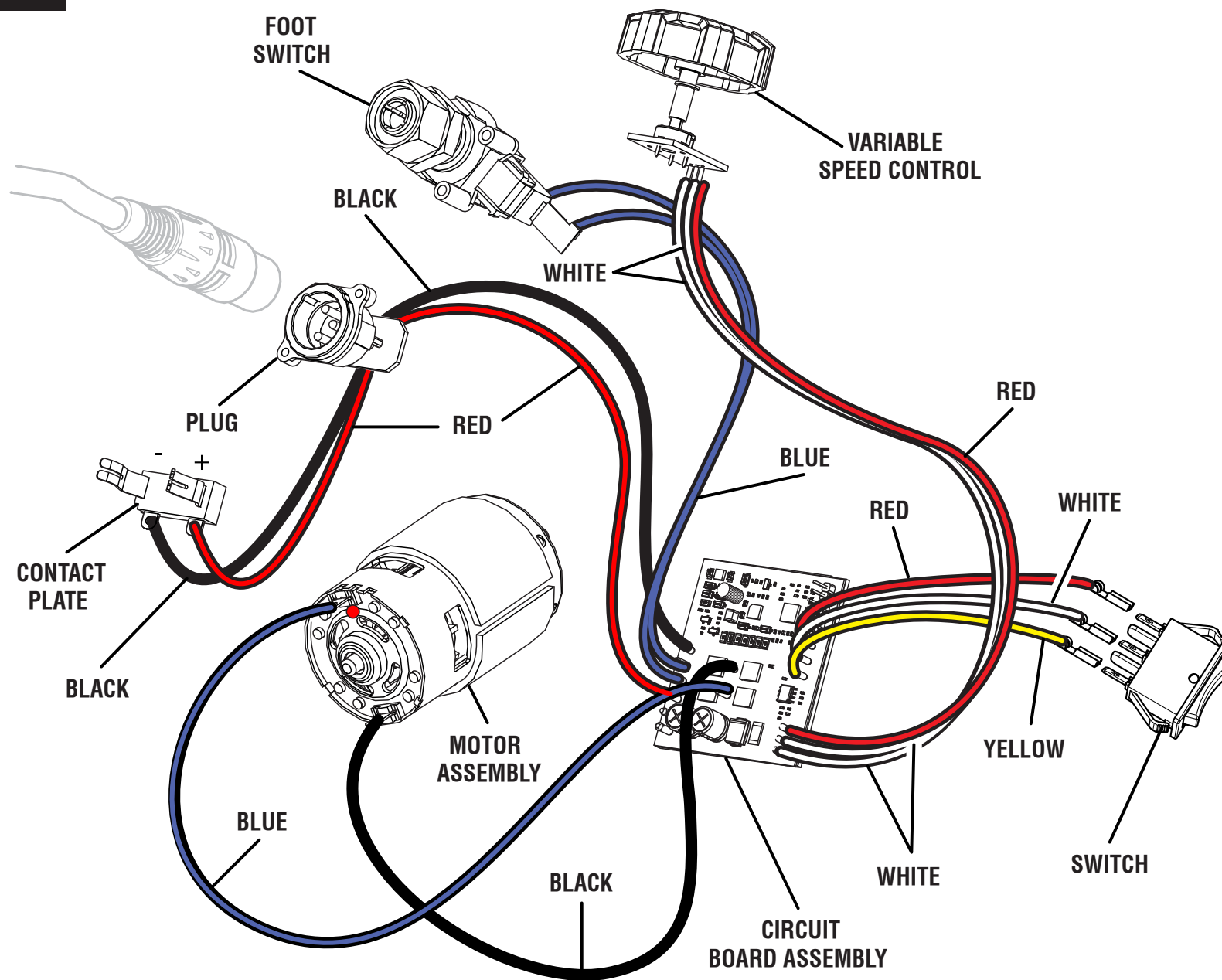
WIRING DIAGRAM
