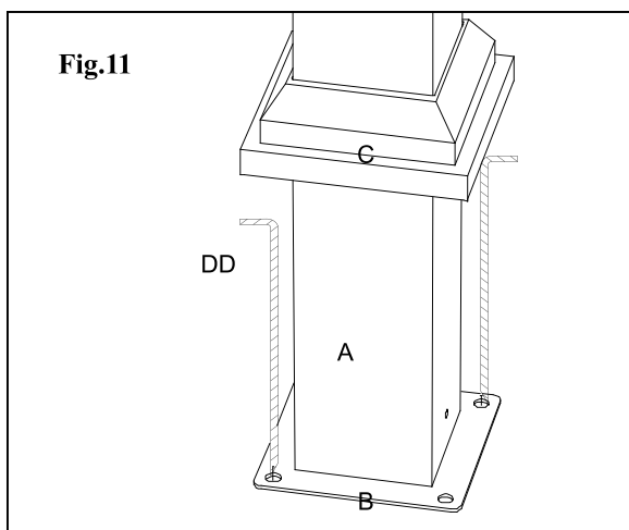
Fig.11: Attach the assembled pergola to lawn with Stake (DD).
