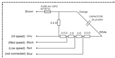
Motor wiring sketch
