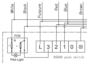
Switch assembly
