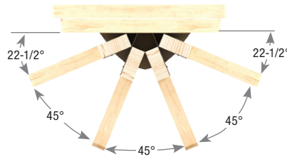
BN264 Standard configuration (top view)
