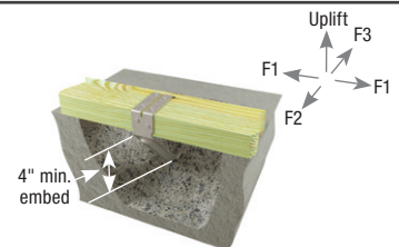
Typical FA3 standard installation in concrete
