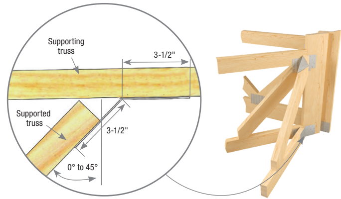
Alternate SNP3 installation Figure 2
