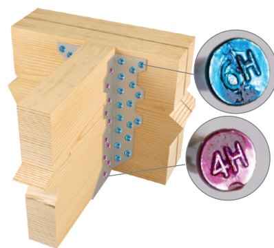
Typical MiTek hanger installation using TECO 33° Collated Nails
