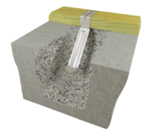
Alternate FA3 installation
