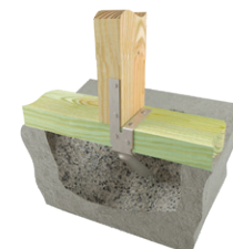
Typical FA3 one-tab-up installation
