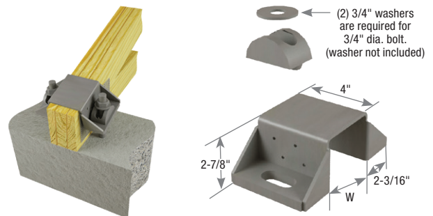
Typical HUGT2 installation
