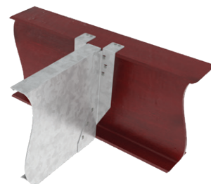
Typical HDOL/S1616 (I-beam) installation
