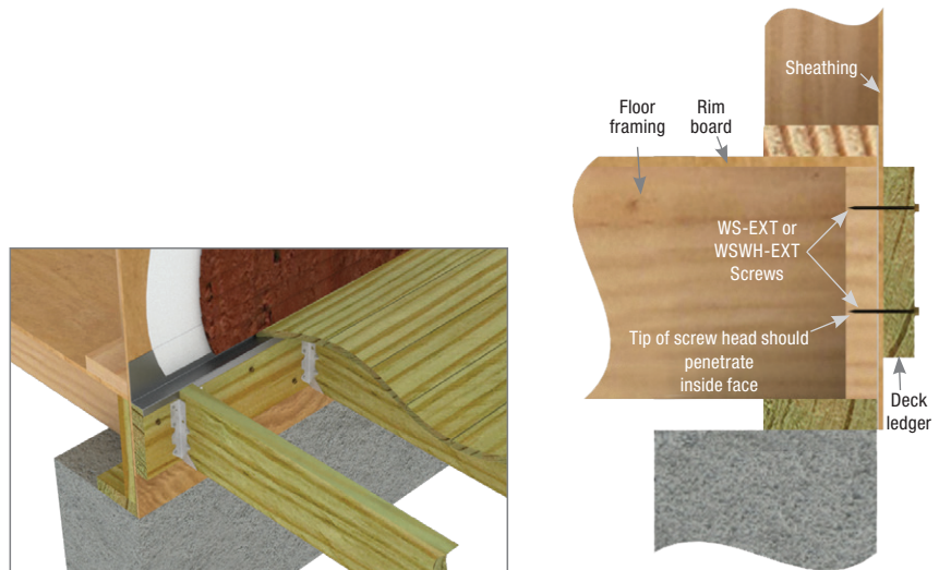
Perspective view
