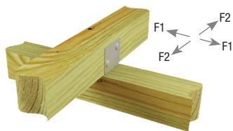
Typical TTU2-TZ installation
