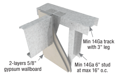
Typical FWH/S deep-track installation Figure 2
