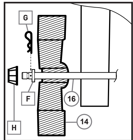
ASSEMBLED VIEW
