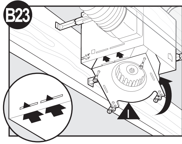
B23 Reinstall the motor by inserting the tabs and pushing up into position. Make sure the wires are not pinched between the motor and the housing.
