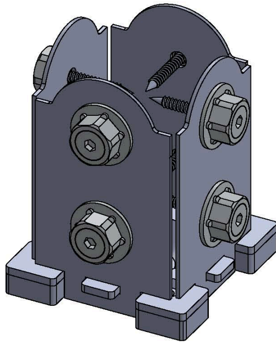
4" x 4" Post Base Kit #56607
