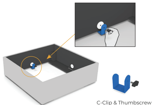
C-Clip & Thumbscrew
