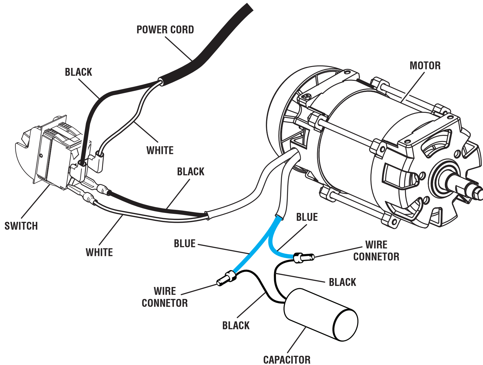
WIRING DIAGRAM
