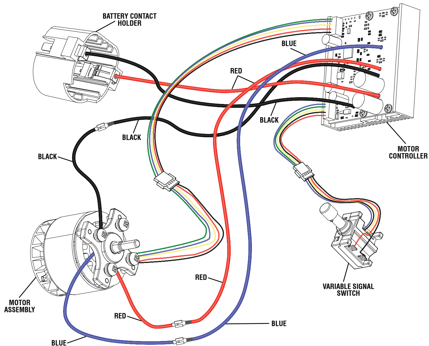
WIRING DIAGRAM
