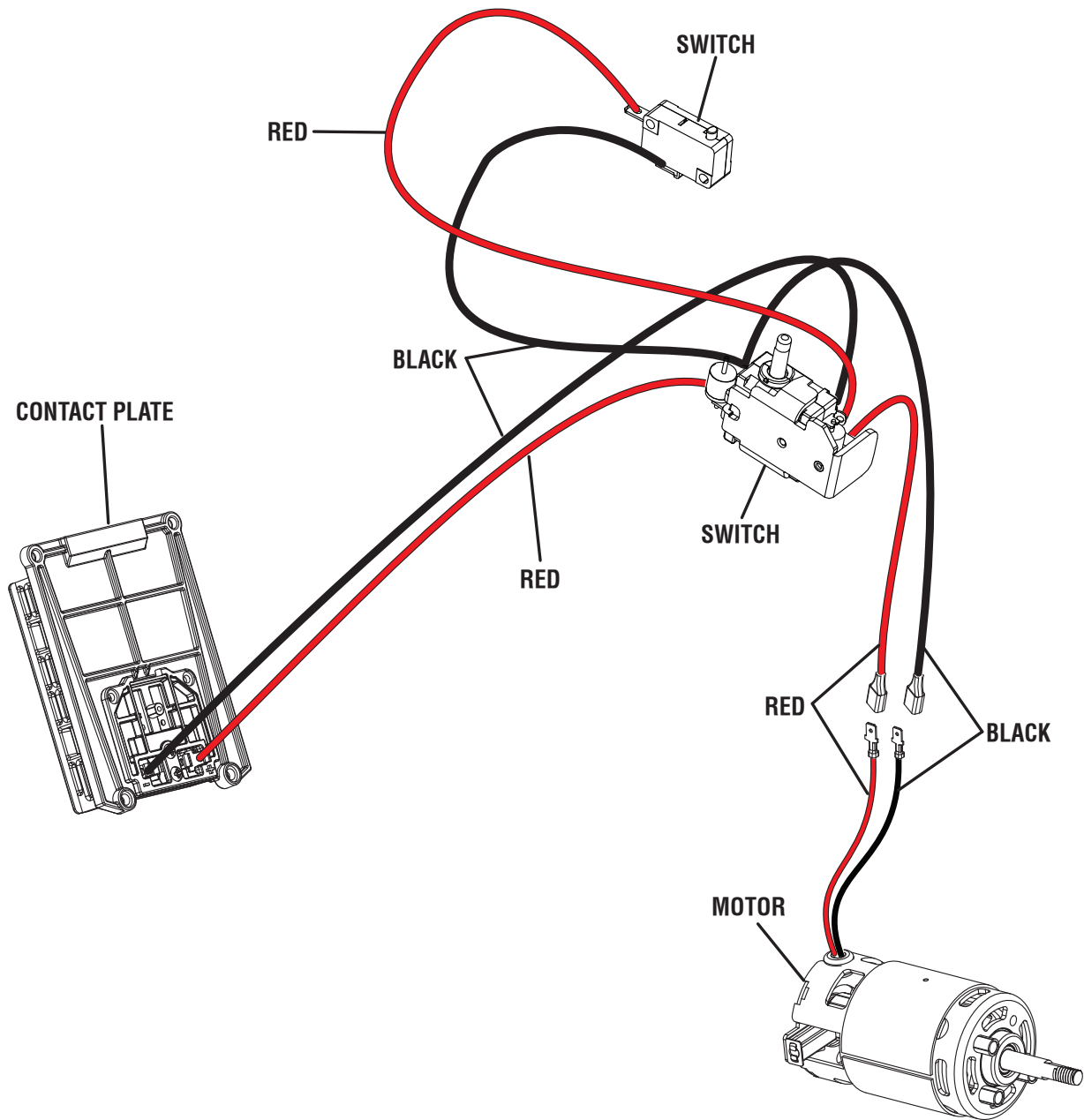
WIRING DIAGRAM
