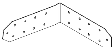
A4M01302 (x2) | LEFT OUTSIDE BRACKET
