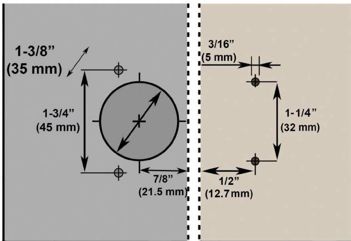
Face Frame Cabinet Door (Cup of hinge)
