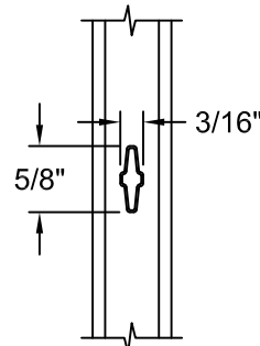
5/8" Contour GBG
