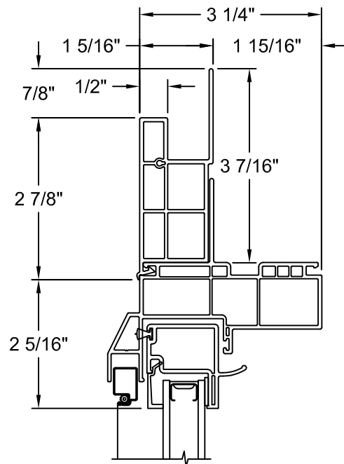
Flat Casing
