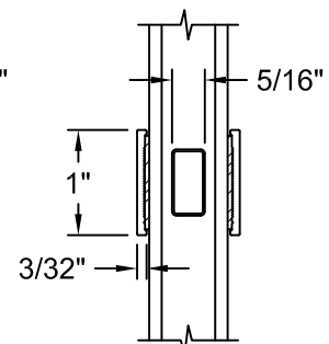
1" Flat SDL
