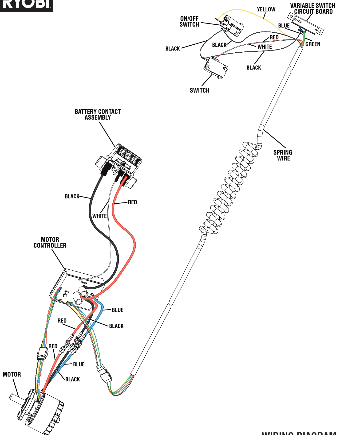
WIRING DIAGRAM
