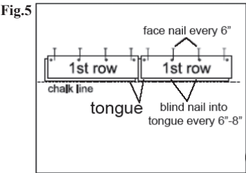
Fig.5 Installing the first rows. Select very straight boards to use in the first rows. The groove side should be facing the wall. At least the first two rows will have to be face & blind nailed as there will not be enough clearance to use the flooring nailer. At the end of the first row, put a 3/4" spacer along the wall, measure the length of the last plank to fit and cut.
