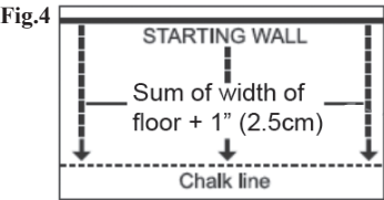
Establish a straight line by measuring a point out from the starting wall in at least three places equal to the width of the flooring face, plus 1/4" for the tongue and 3/4" for the expansion space. Snap a chalk line.
