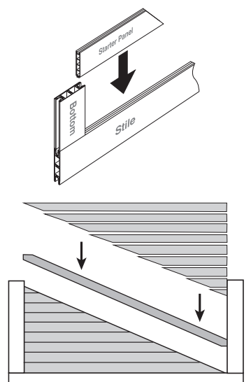
Figure 8 Starter Panel This side into Stile Channel
