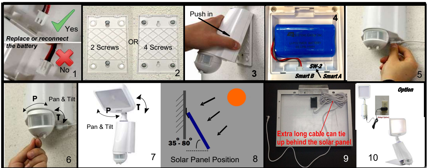
Fig. 1 Installation Steps
