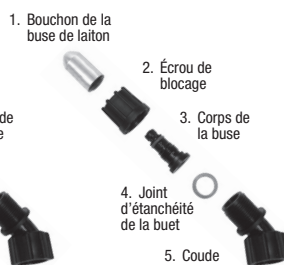
Figure 2 Buse de laiton ajustable
