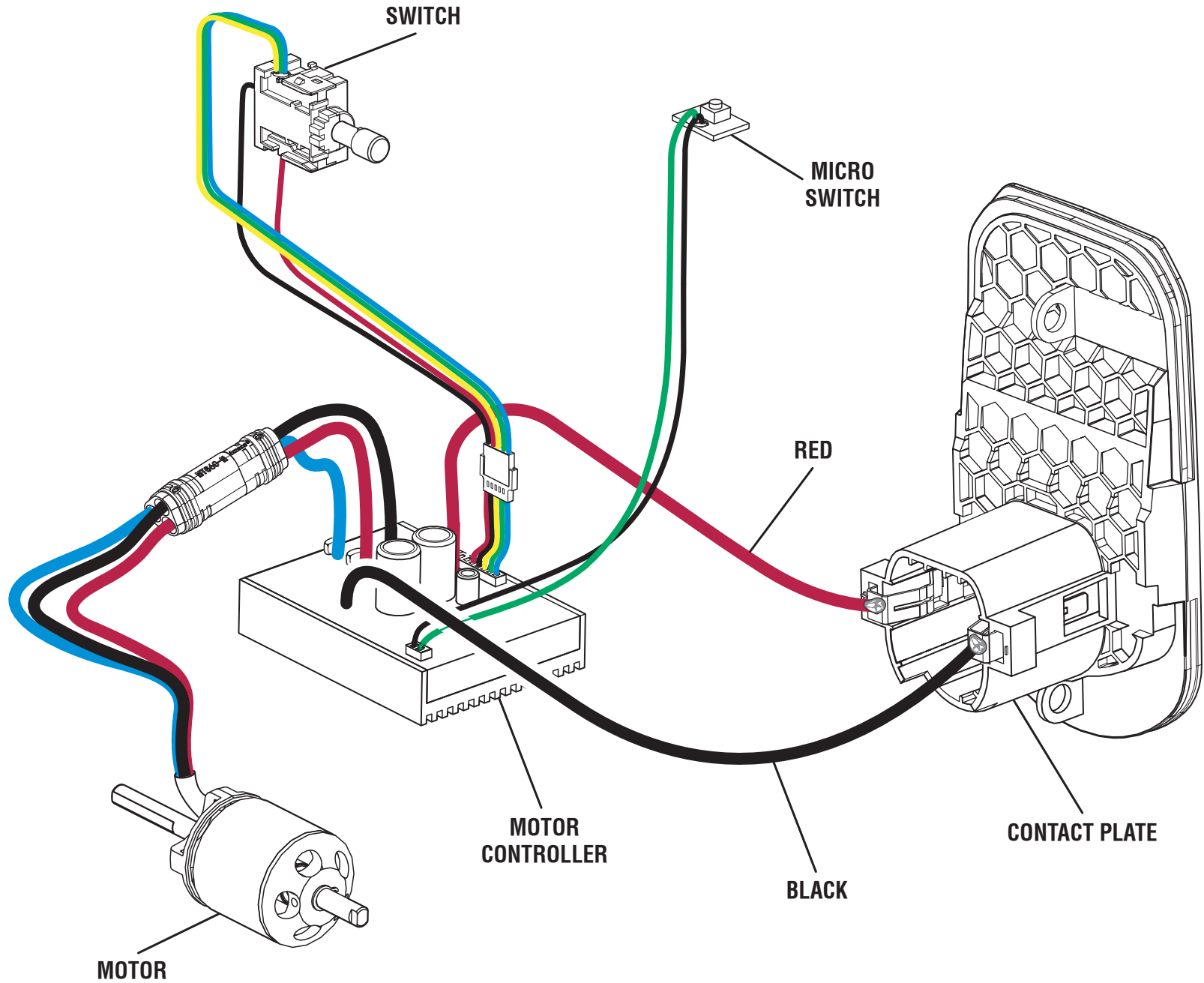
WIRING DIAGRAM
