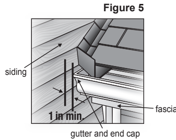
Figure 5 Maintain a minimum 1 in gap between gutter end caps and siding & trim.
