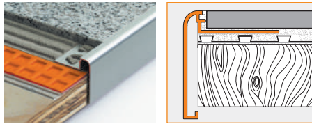
2.8 Schluter®-RODEC-STEP
