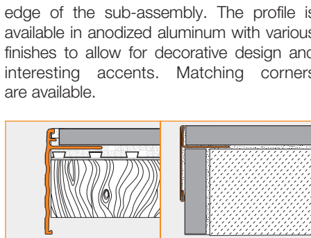
3.4 Schluter®-TREP-FL
