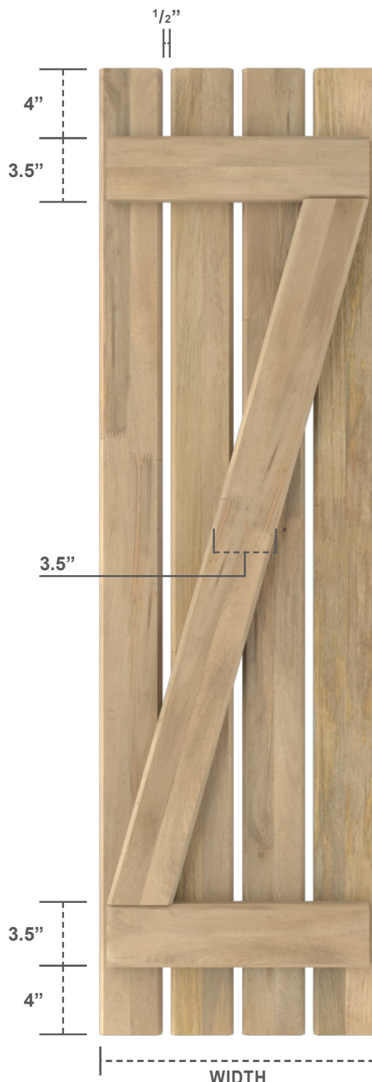
FRONT VIEW
