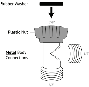
Hybrid Cold Water T-Adapter (7/8" x 7/8" x 1/2") SKU: HybridT1516
