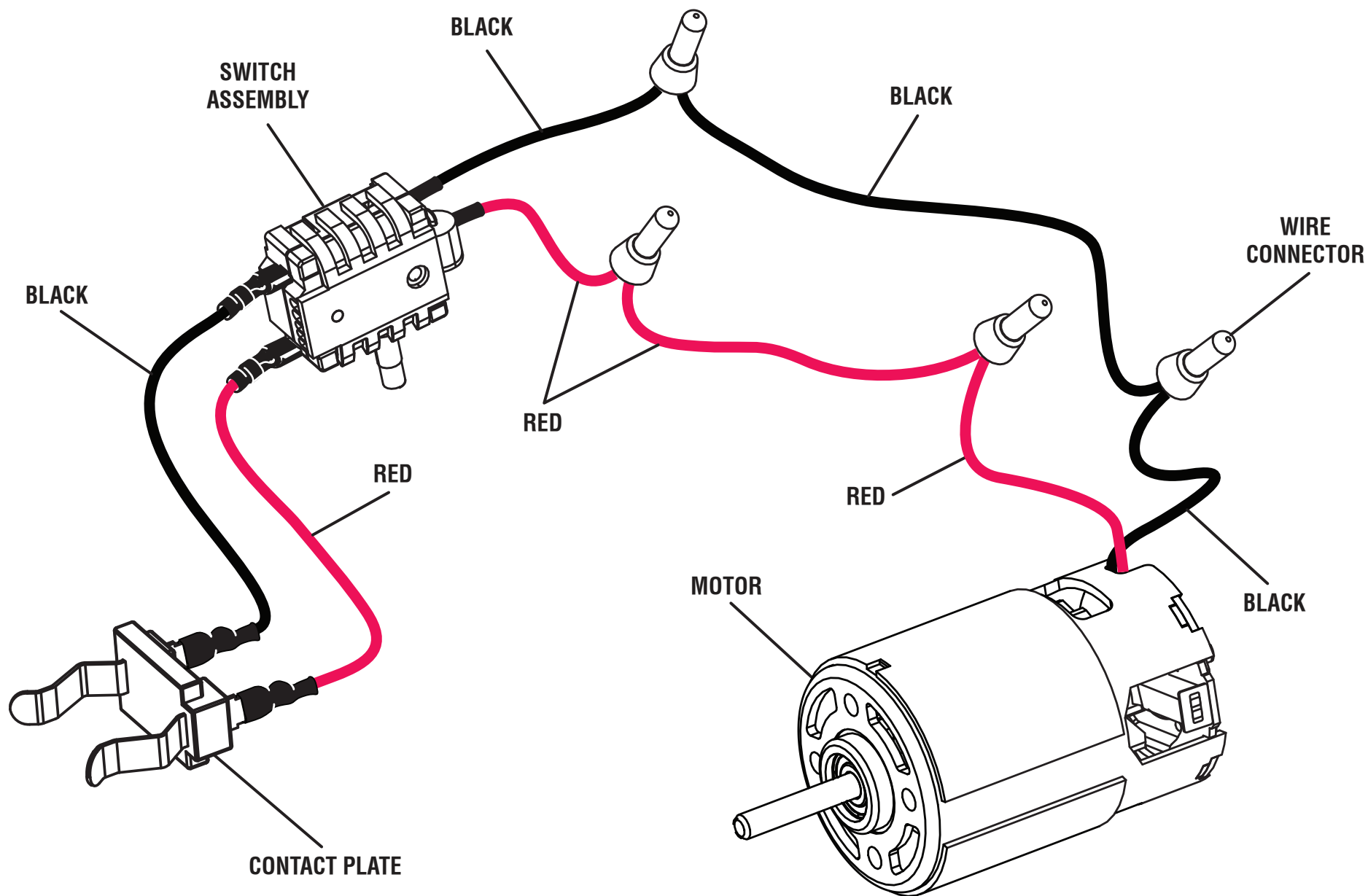
WIRING DIAGRAM
