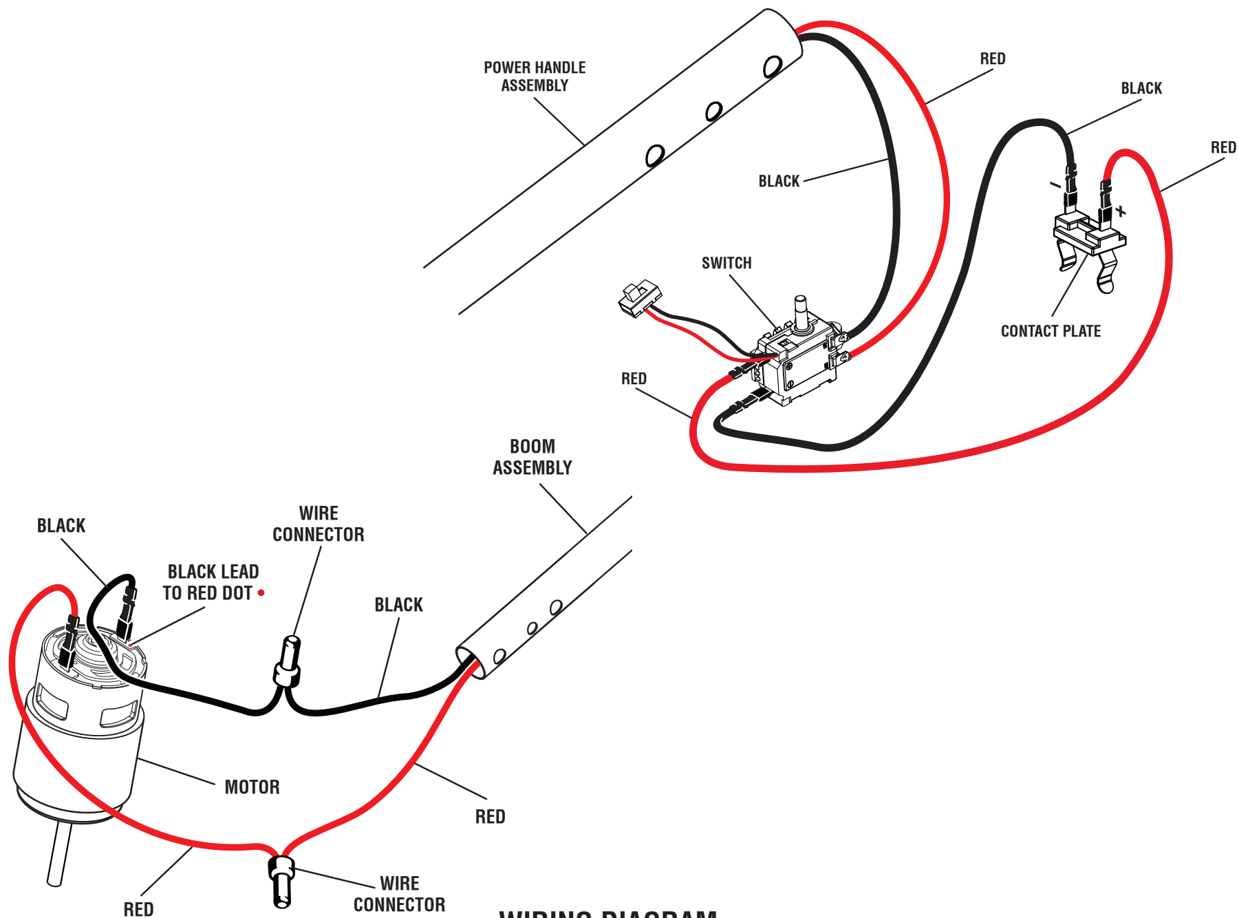
WIRING DIAGRAM
