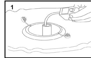
1 Insert water pump cable through the opening
