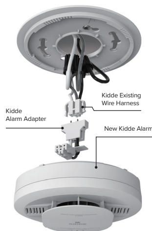
FIGURE 2: Adapter connecting to the old harness
