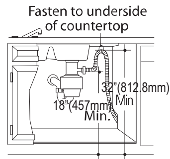
Disposer Installation
