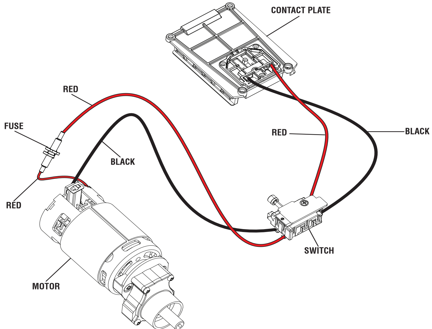
WIRING DIAGRAM
