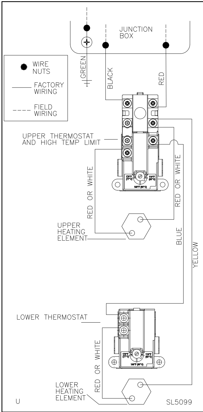
Figure 6 - Dual Element Model Wiring Detail, Non-Simultaneous Element Operation - Green Wire for Grounding the Water Heater
