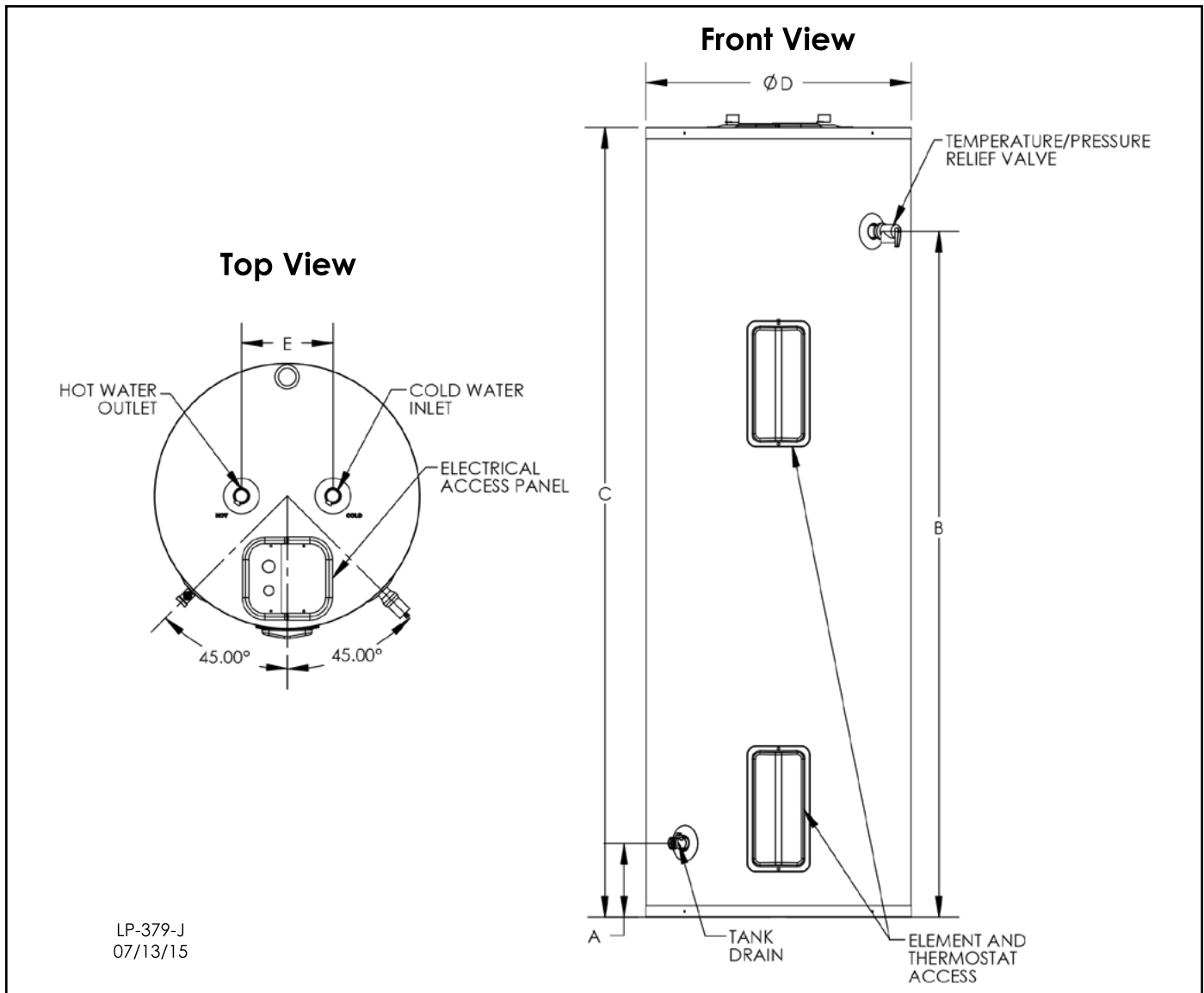
Figure 2 - Dimensional Drawing - Non-Simultaneous Operation
