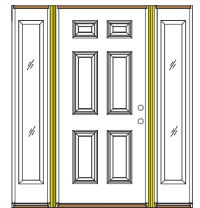
Box construction with spread mullion
