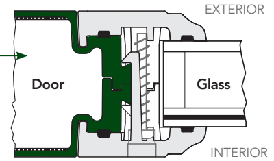
Flush Glaze Frame
