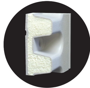
Heavy duty molded panels feature a structural foam core for added strength and rigidity
