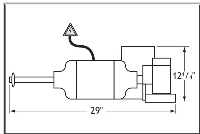
Figure 4. Machine clearances.
