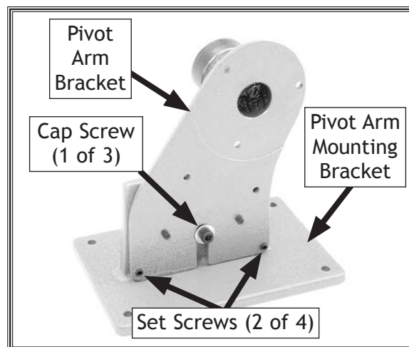
Figure 8. Left side of pivot arm bracket assembly.
