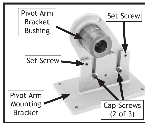
Figure 9. Right side of pivot arm bracket assembly.
