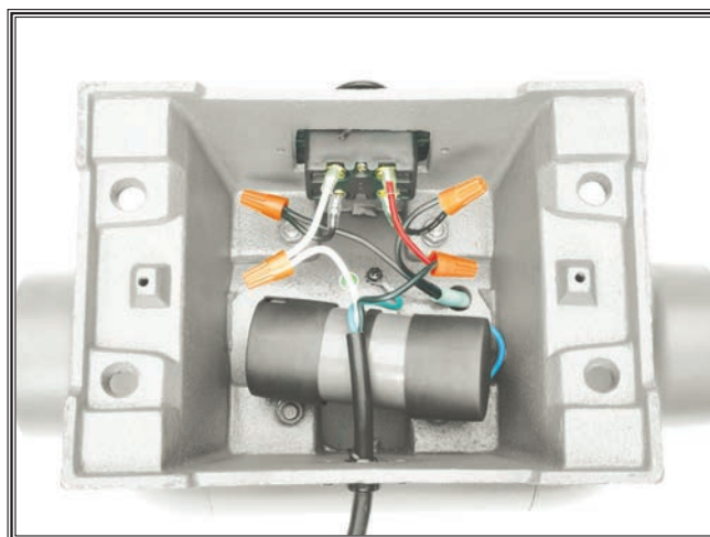
Figure 33. Electrical wiring.
