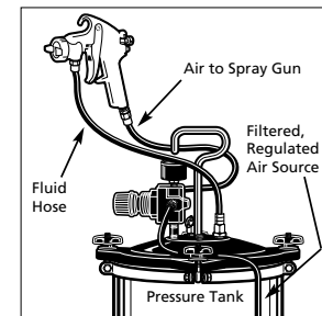
Figure 4 - Pressure Feed Tank Set-up
