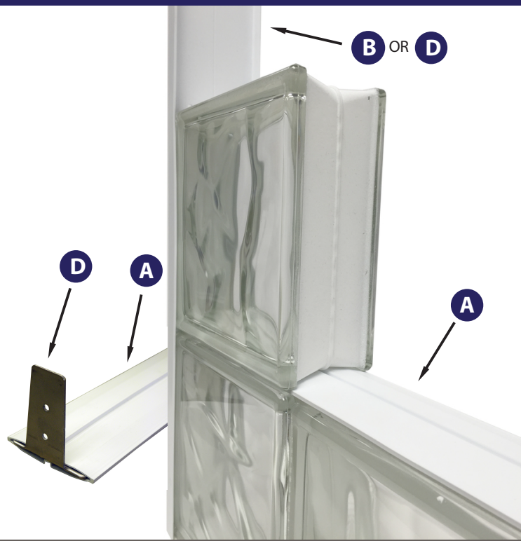
B Perimeter Channel Model #: VCHAN3
