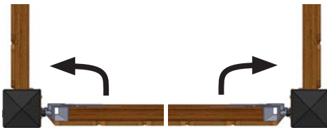
Left Swing Perpendicular Installation
