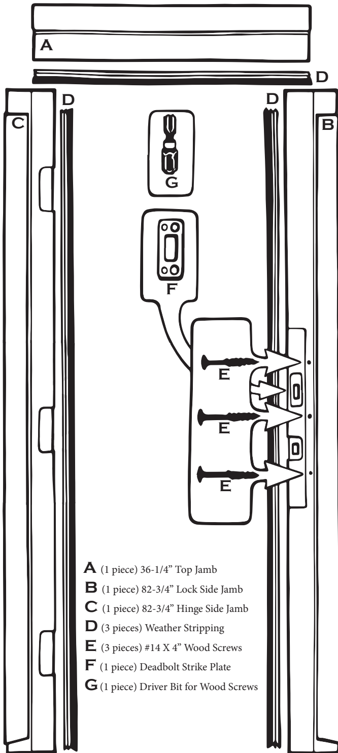
LEFT HAND INSWING VIEWED FROM EXTERIOR
