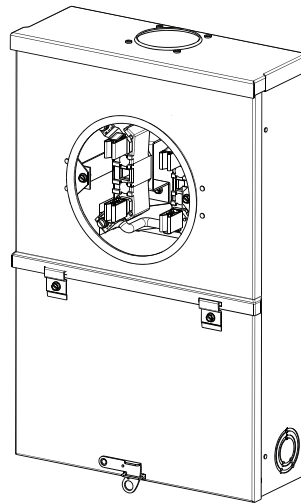
Surface Mount (JA1020B1100S)
