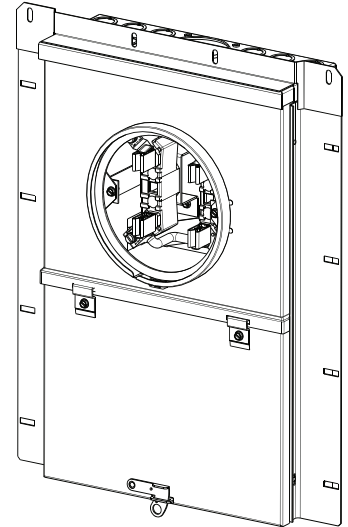
Flush Mount (JA1020B1100F)
