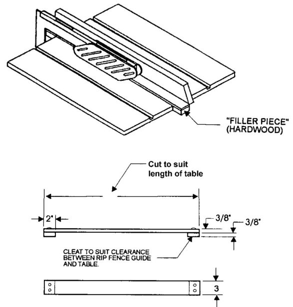
Figure 45 – Filler Piece
